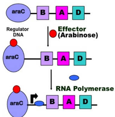
original ara Operon
