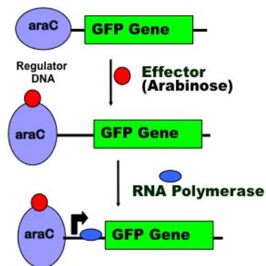
modified ara Operon
